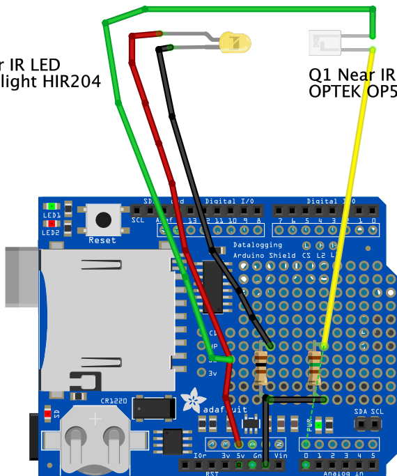
WATER CLARITY SENSOR ELECTRONICS LAYOUT
