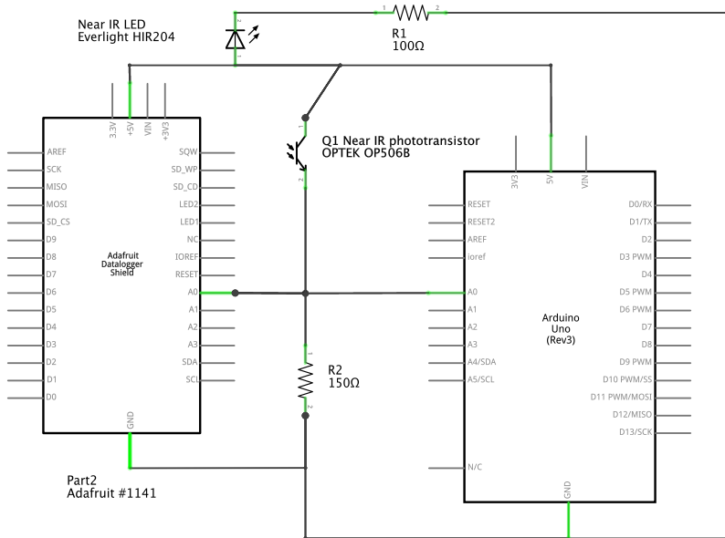
WATER CLARITY SENSOR SCHEMATIC fritzing
